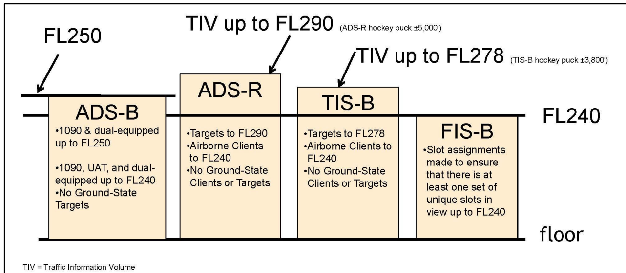
FIG 4-5-10 Terminal – ADS-B/ADS-R/TIS-B/FIS-B Service Ceilings/Floors
