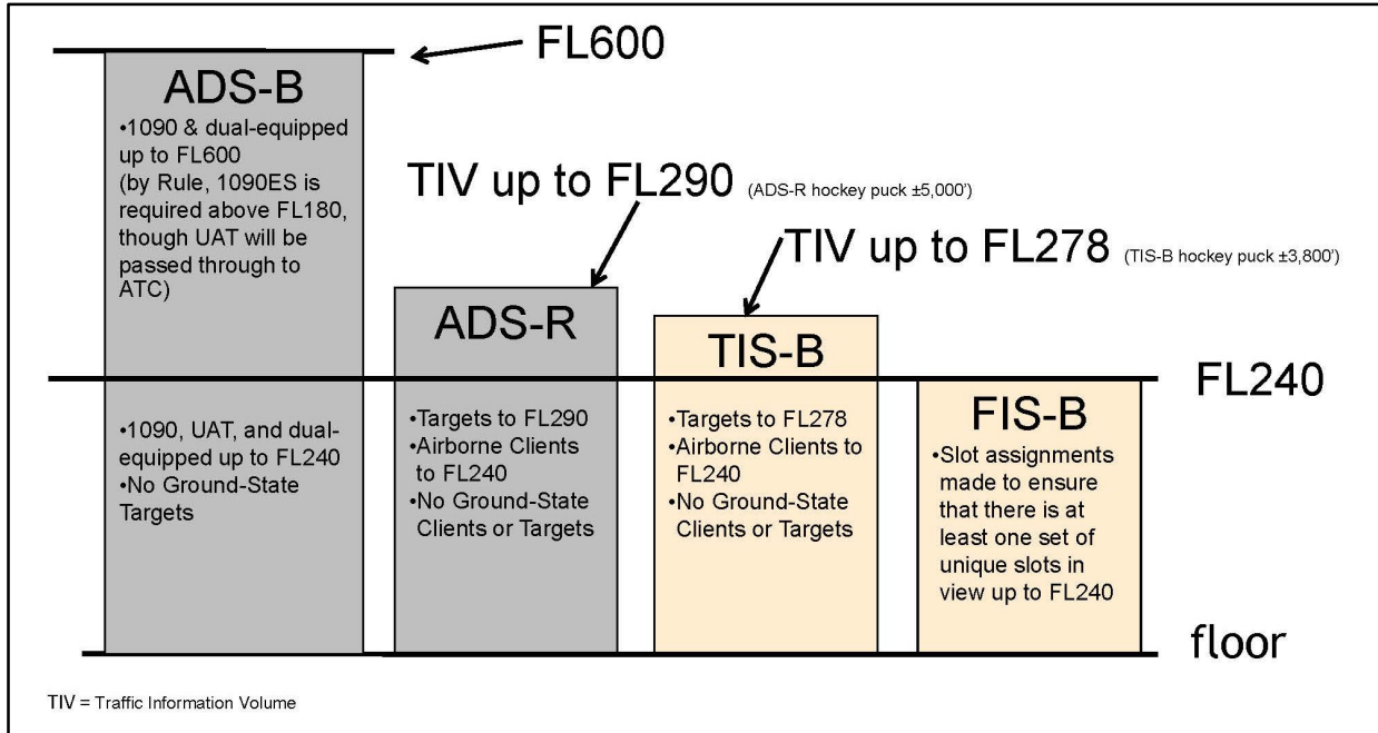
FIG 4-5-9 En Route – ADS-B/ADS-R/TIS-B/FIS-B Service Ceilings/Floors
