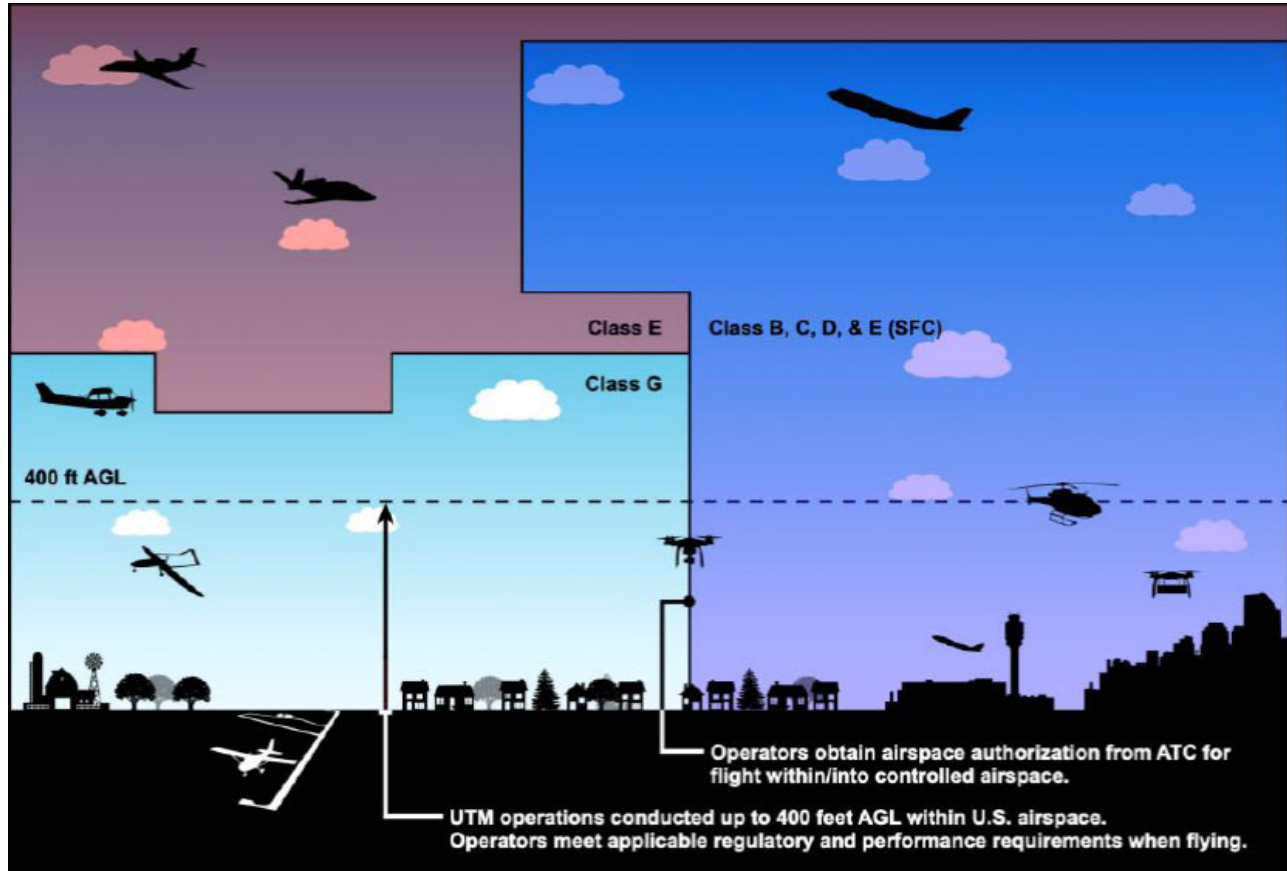
FIG II-4-2 UTM Operations in Context of Airspace Classes
